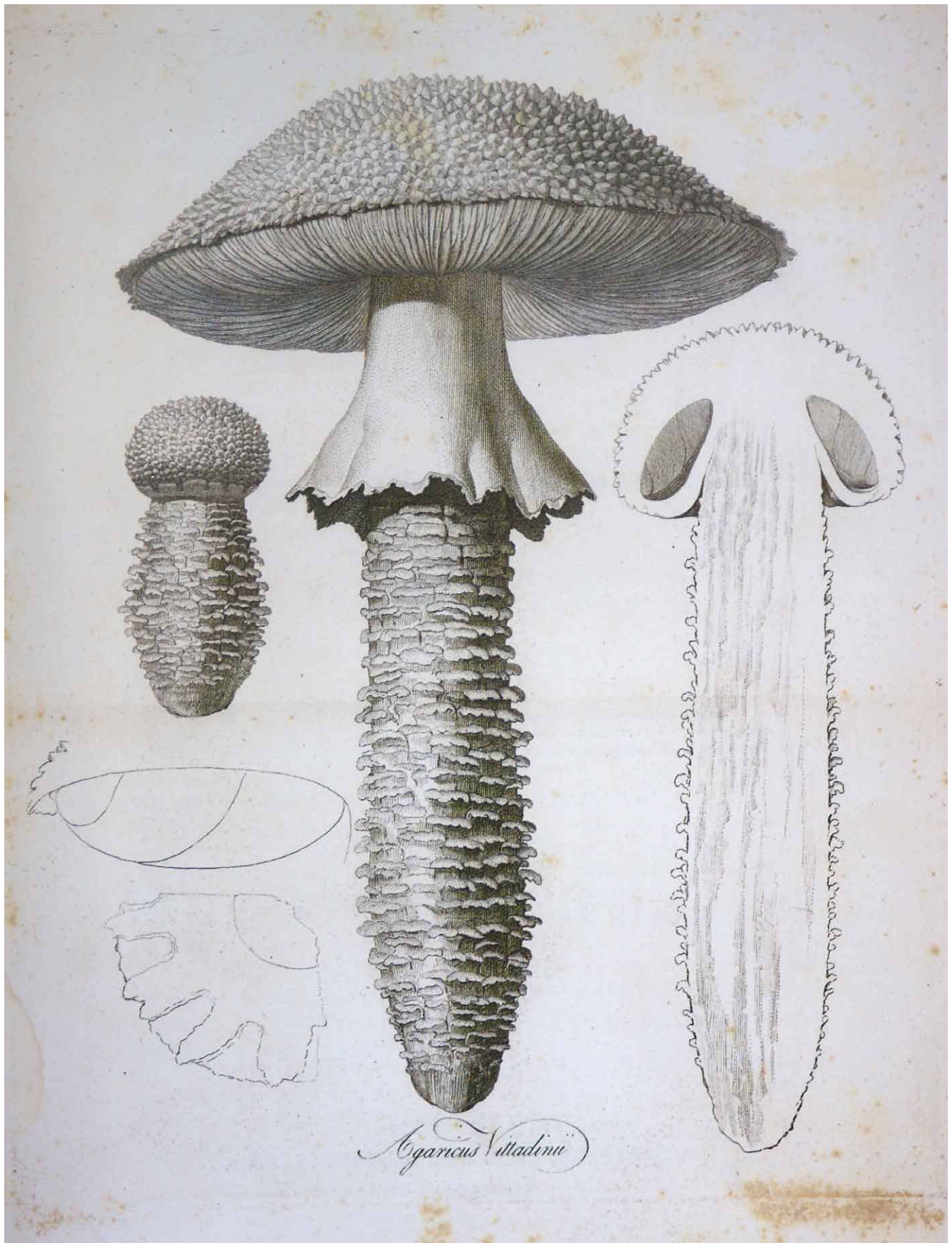
Fig. 1. Agaricus vittadini illustrated by Moretti (1826b: tab. 1 – selected as lectotype by Bas) and reproduced in Vittadini (1826).
